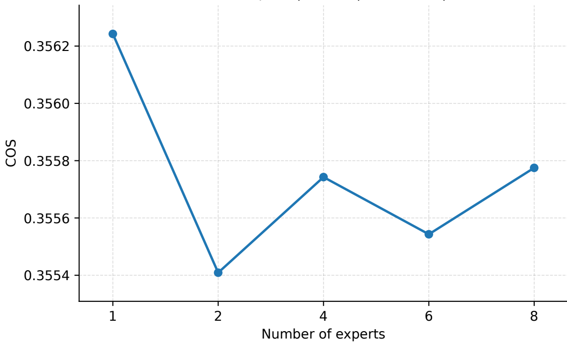
Number of Experts | Seattle | PredLen=5 | COS
