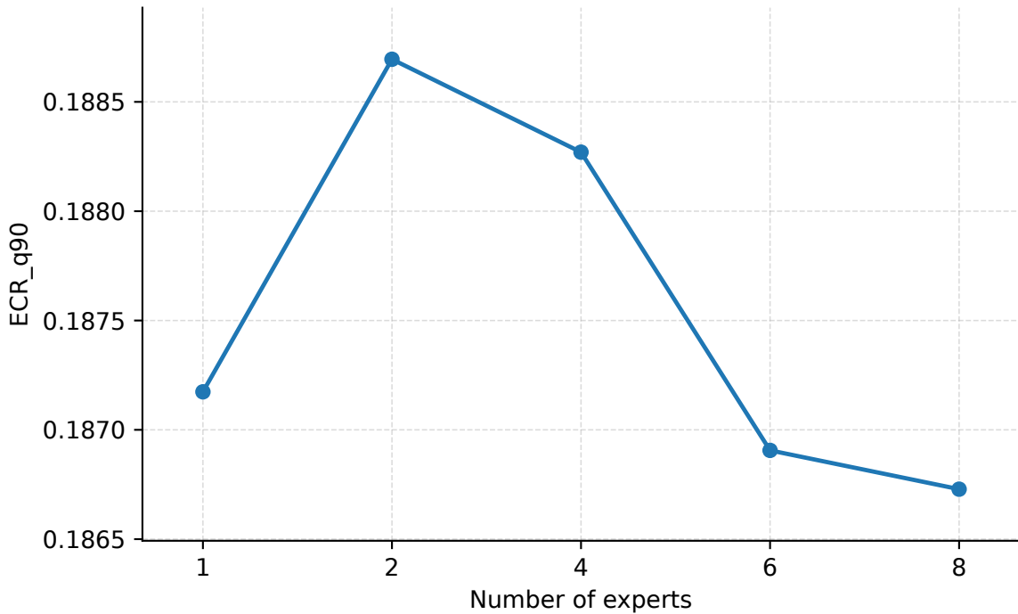
Number of Experts | Seattle | PredLen=5 | ECR_q90
