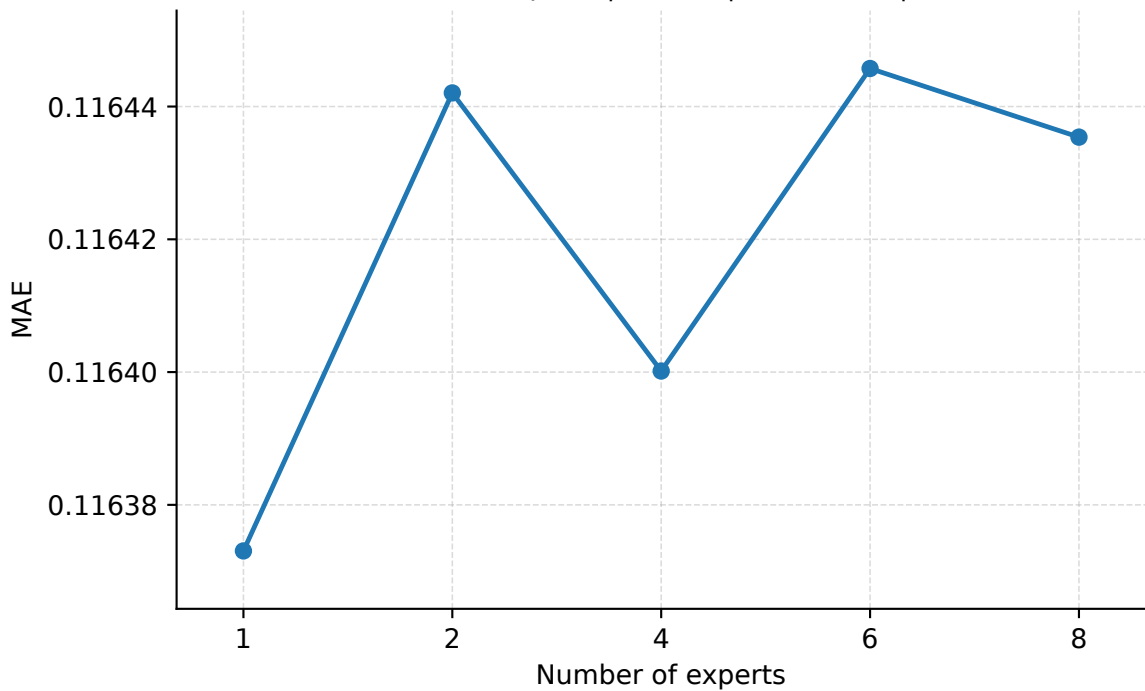
Number of Experts | Seattle | PredLen=5 | MAE
