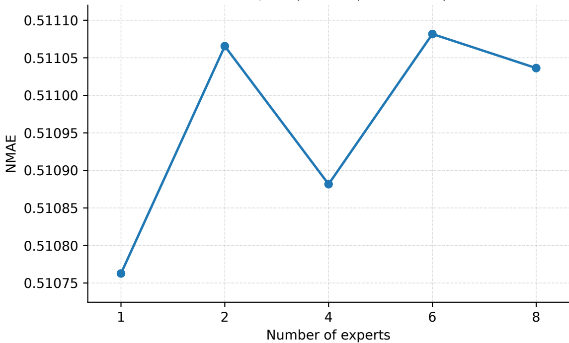
Number of Experts | Seattle | PredLen=5 | NMAE
