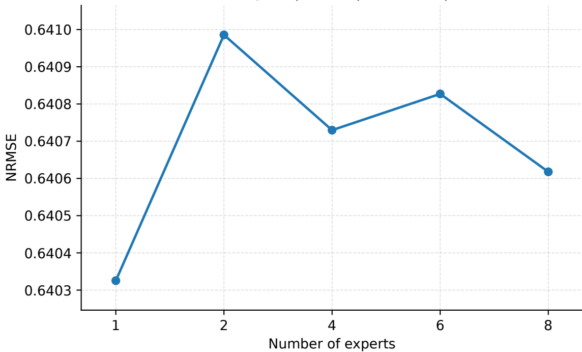
Number of Experts | Seattle | PredLen=5 | NRMSE
