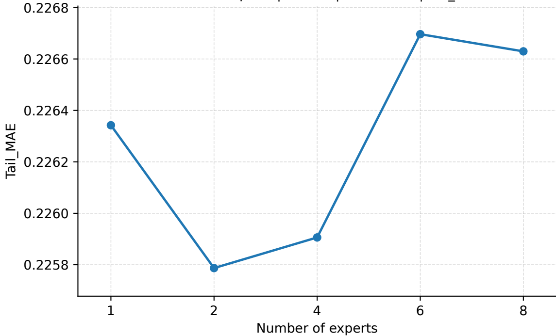
Number of Experts | Seattle | PredLen=5 | Tail_MAE
