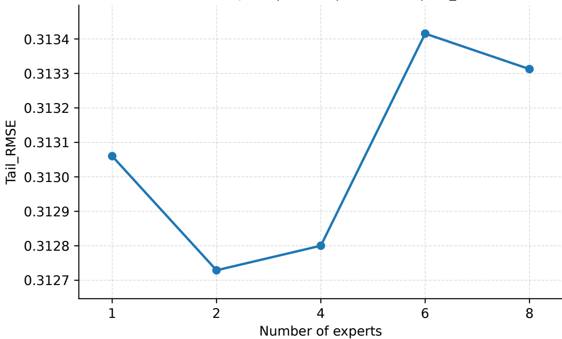
Number of Experts | Seattle | PredLen=5 | Tail_RMSE
