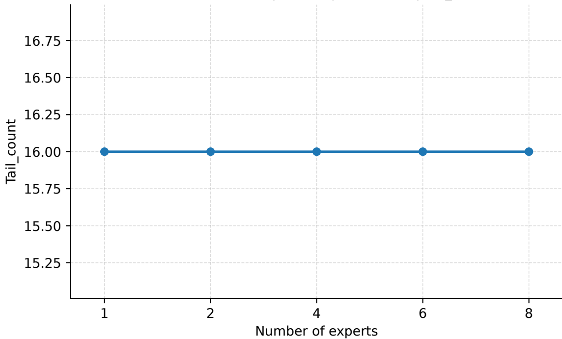
Number of Experts | Seattle | PredLen=5 | Tail_count
