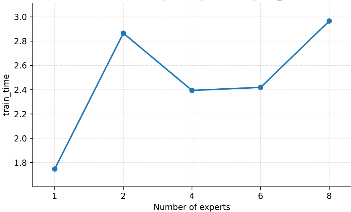
Number of Experts | Seattle | PredLen=5 | train_time
