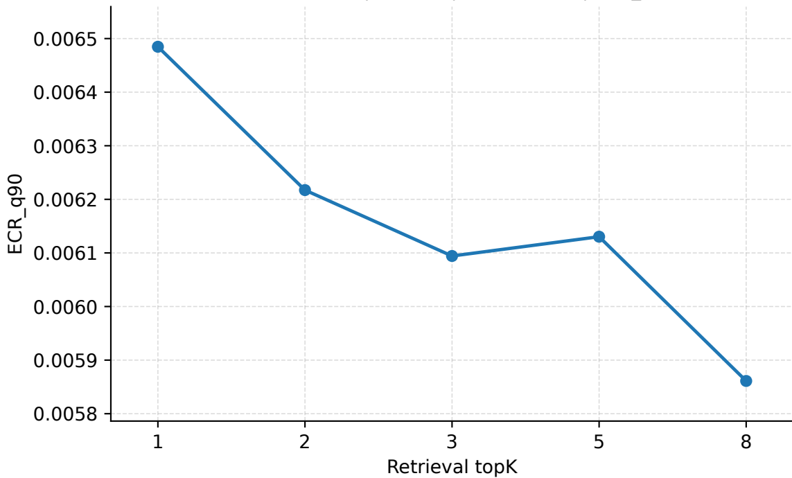
Retrieval topK | Abilene | PredLen=10 | ECR_q90
