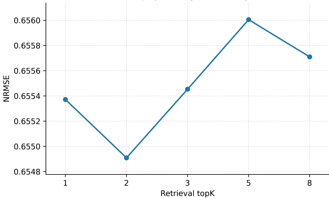
Retrieval topK | Abilene | PredLen=10 | NRMSE
