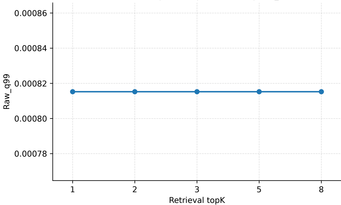
Retrieval topK | Abilene | PredLen=10 | Raw_q99
