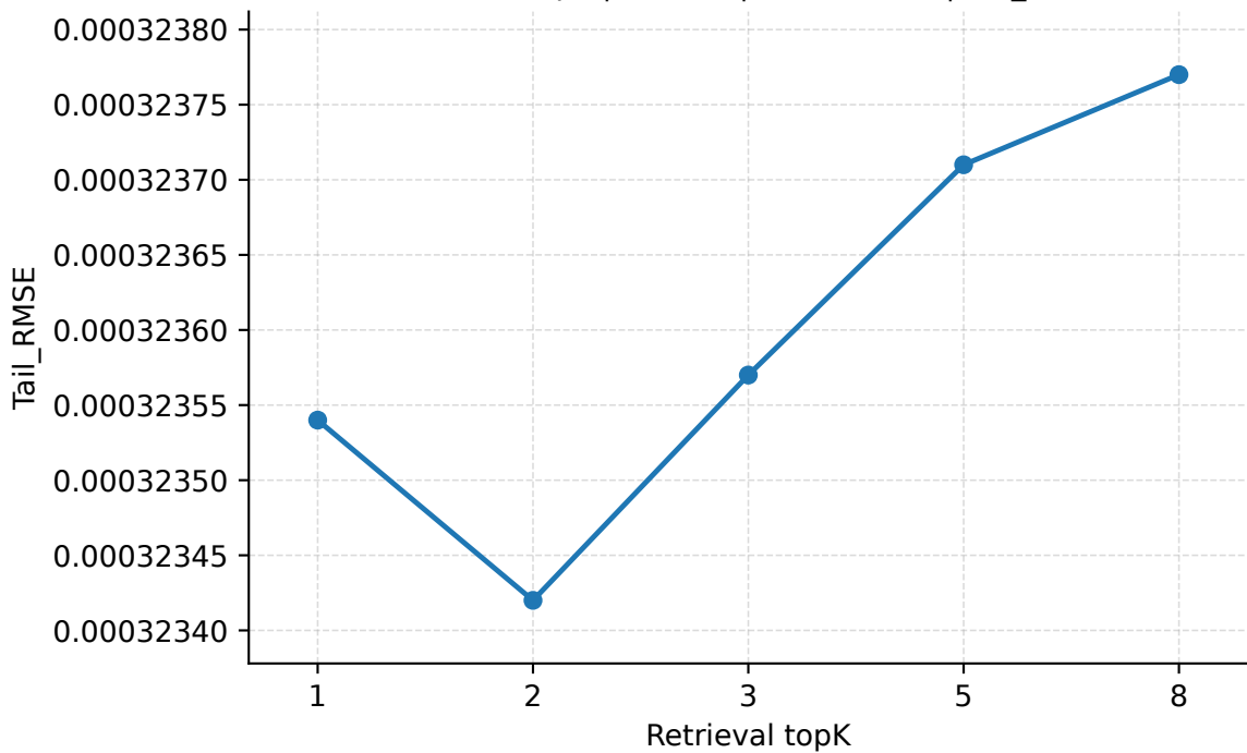
Retrieval topK | Abilene | PredLen=10 | Tail_RMSE
