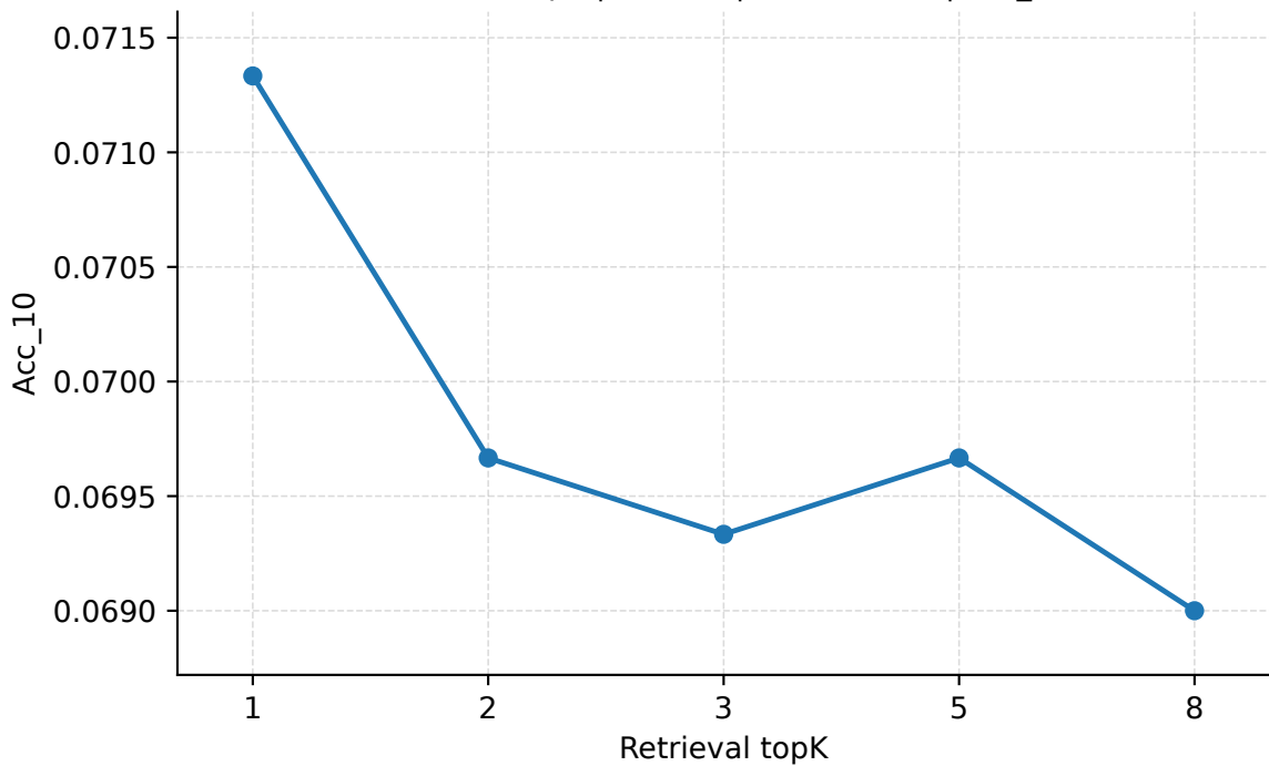
Retrieval topK | Abilene | PredLen=15 | Acc_10
