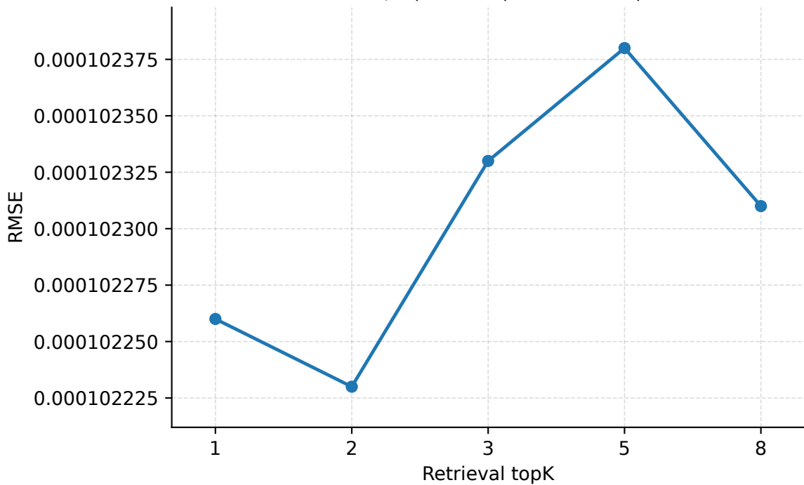
Retrieval topK | Abilene | PredLen=15 | RMSE
