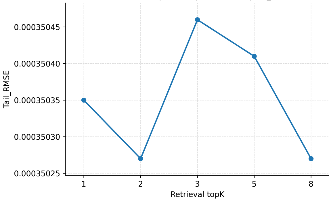
Retrieval topK | Abilene | PredLen=15 | Tail_RMSE
