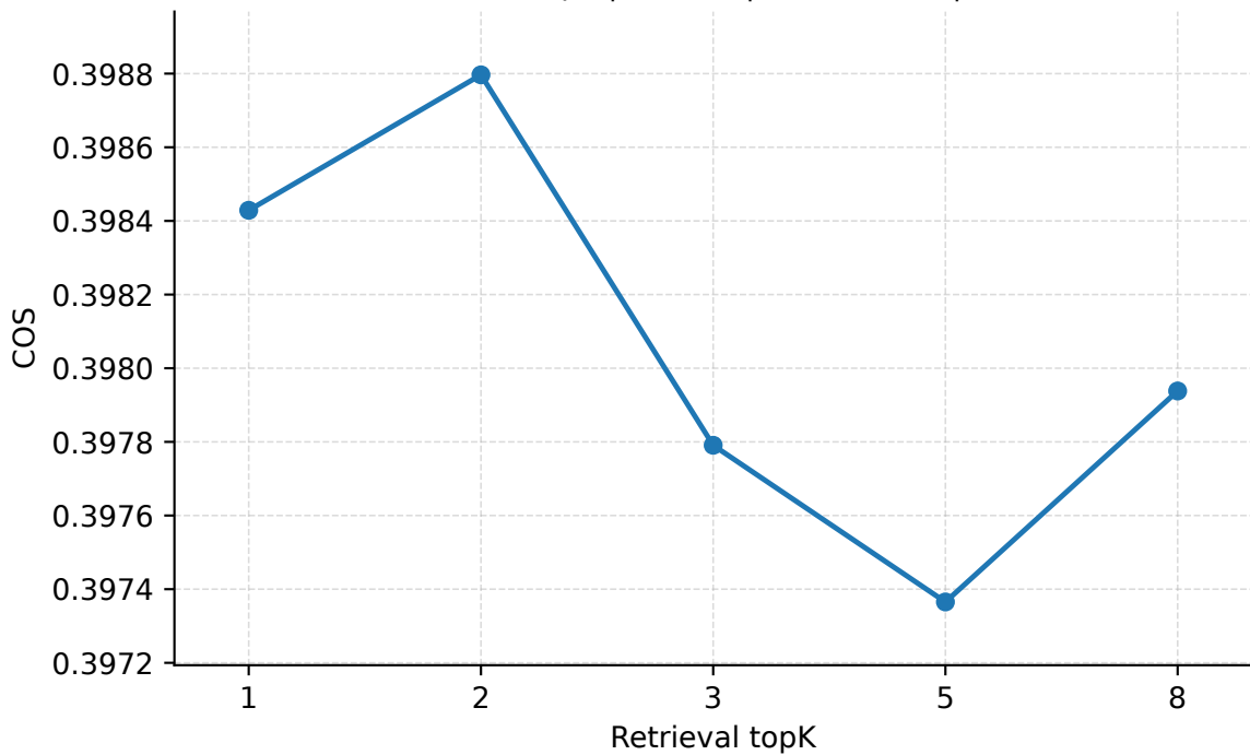
Retrieval topK | Abilene | PredLen=20 | COS
