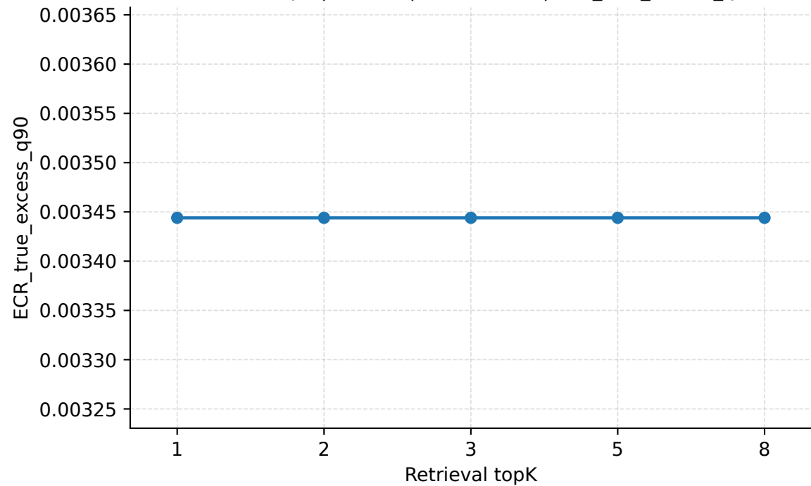
Retrieval topK | Abilene | PredLen=20 | ECR_true_excess_q90
