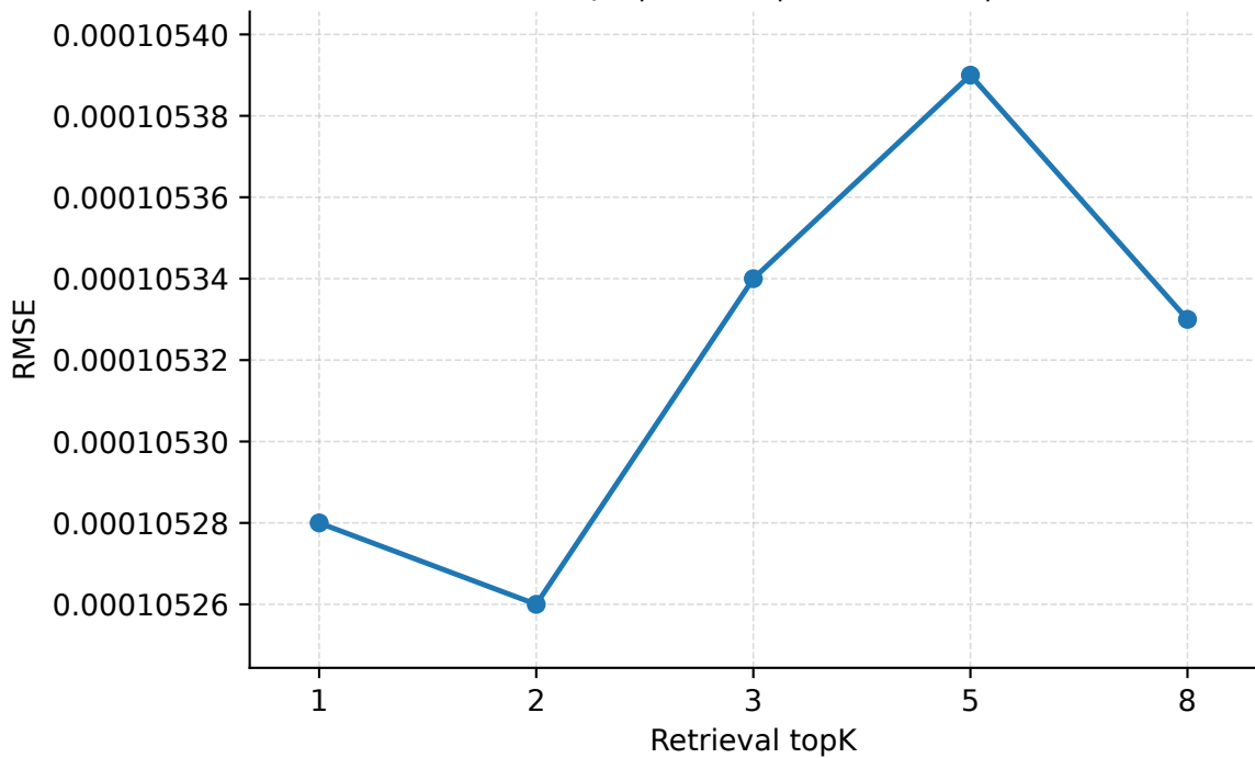
Retrieval topK | Abilene | PredLen=20 | RMSE
