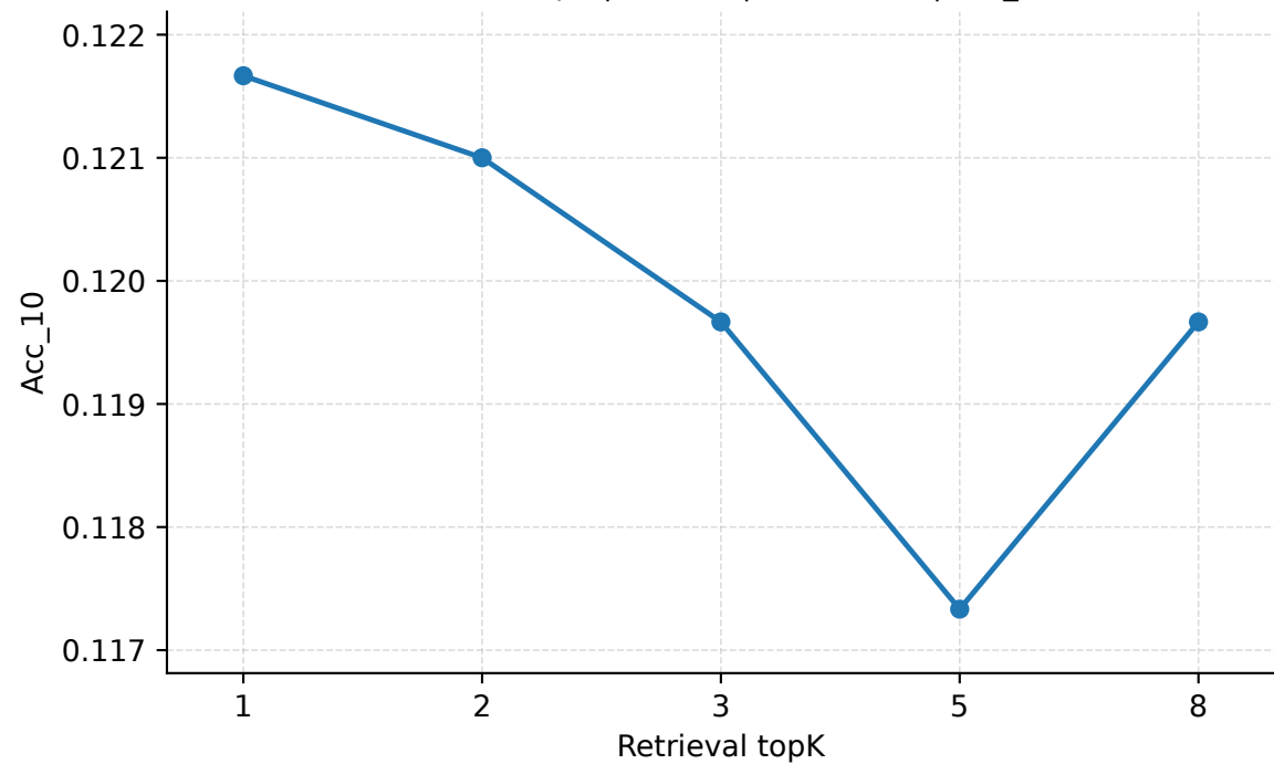
Retrieval topK | Abilene | PredLen=5 | Acc_10
