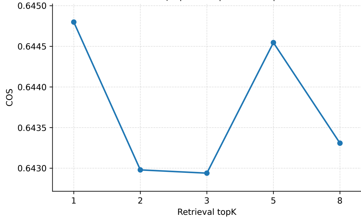
Retrieval topK | Abilene | PredLen=5 | COS
