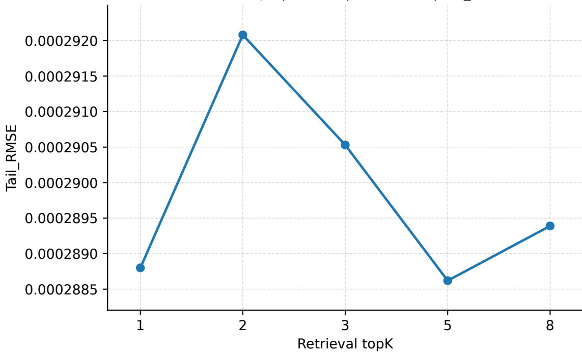
Retrieval topK | Abilene | PredLen=5 | Tail_RMSE
