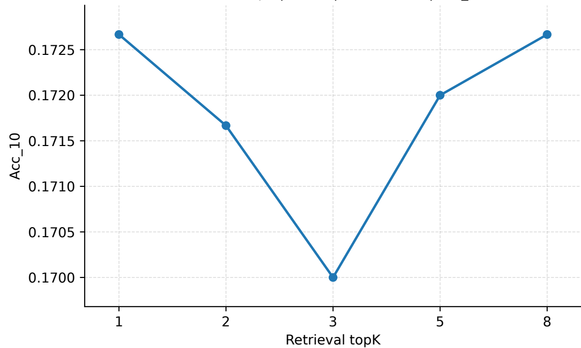
Retrieval topK | Geant | PredLen=10 | Acc_10
