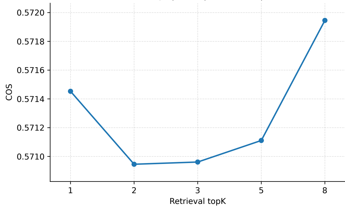
Retrieval topK | Geant | PredLen=10 | COS
