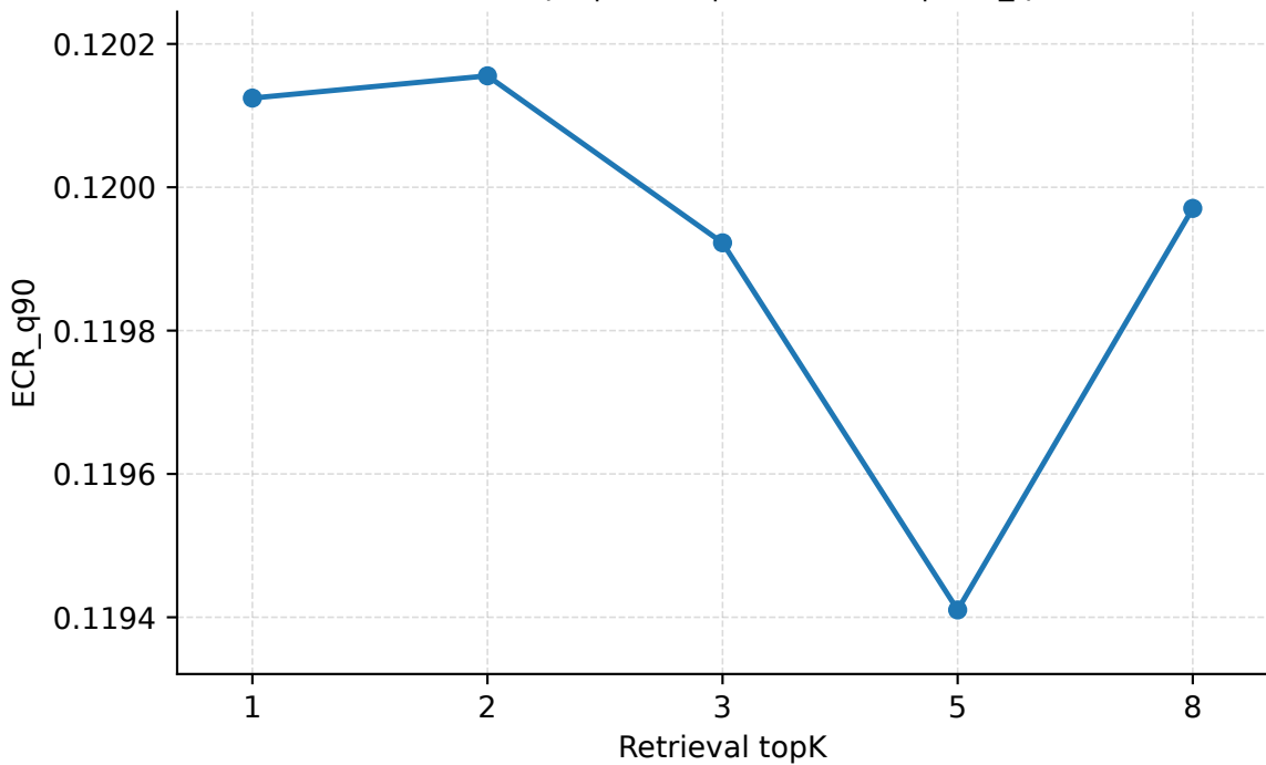
Retrieval topK | Geant | PredLen=10 | ECR_q90
