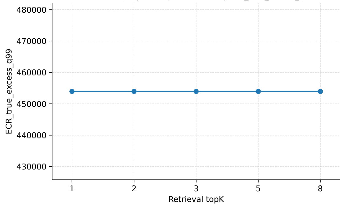
Retrieval topK | Geant | PredLen=10 | ECR_true_excess_q99
