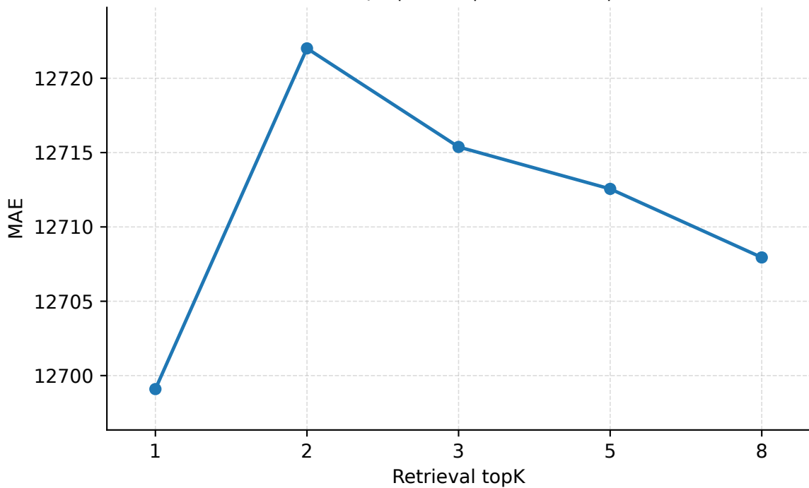
Retrieval topK | Geant | PredLen=10 | MAE
