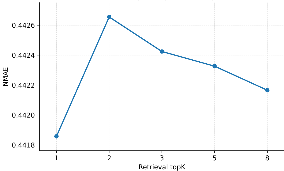
Retrieval topK | Geant | PredLen=10 | NMAE
