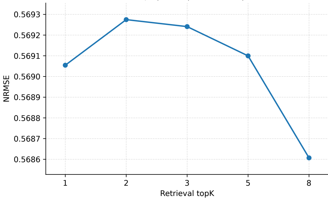
Retrieval topK | Geant | PredLen=10 | NRMSE
