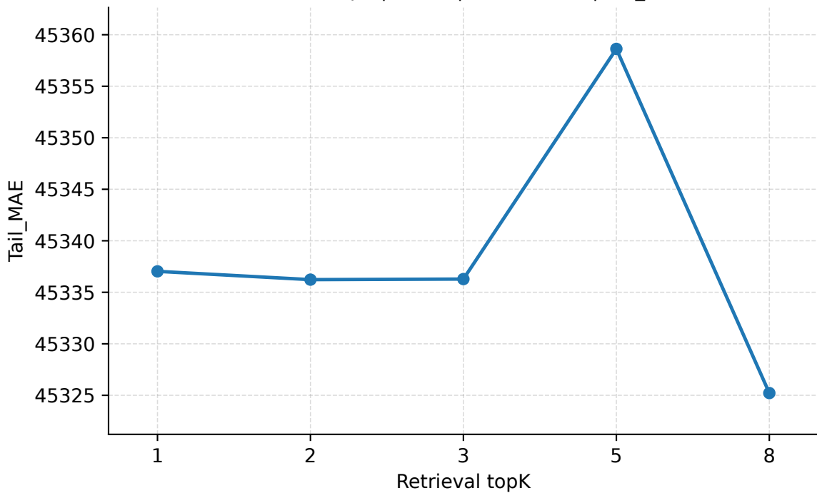
Retrieval topK | Geant | PredLen=10 | Tail_MAE
