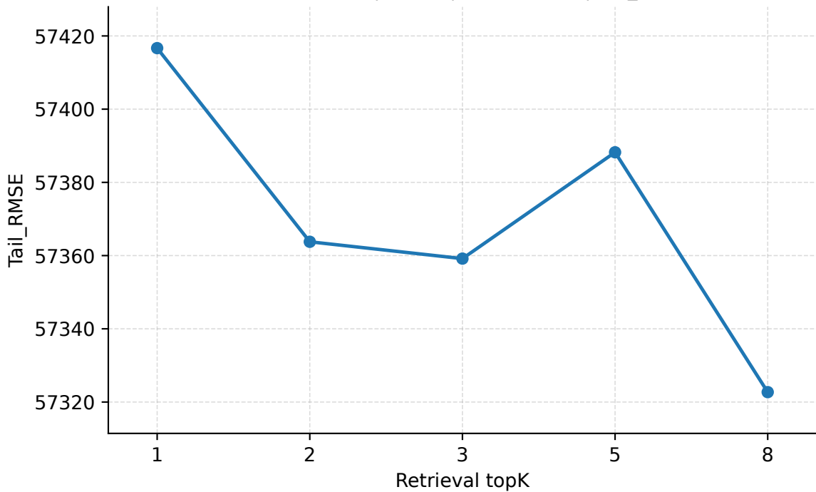
Retrieval topK | Geant | PredLen=10 | Tail_RMSE
