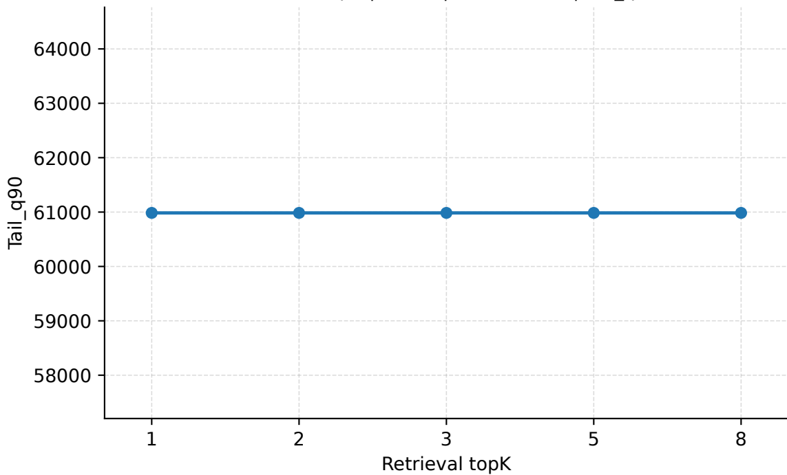
Retrieval topK | Geant | PredLen=10 | Tail_q90
