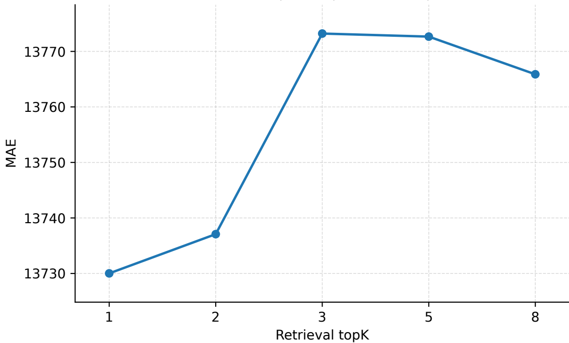
Retrieval topK | Geant | PredLen=15 | MAE
