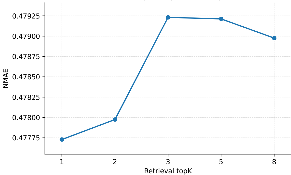
Retrieval topK | Geant | PredLen=15 | NMAE
