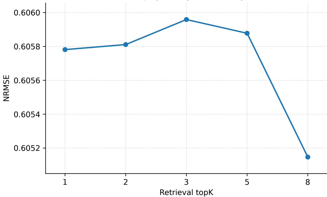
Retrieval topK | Geant | PredLen=15 | NRMSE
