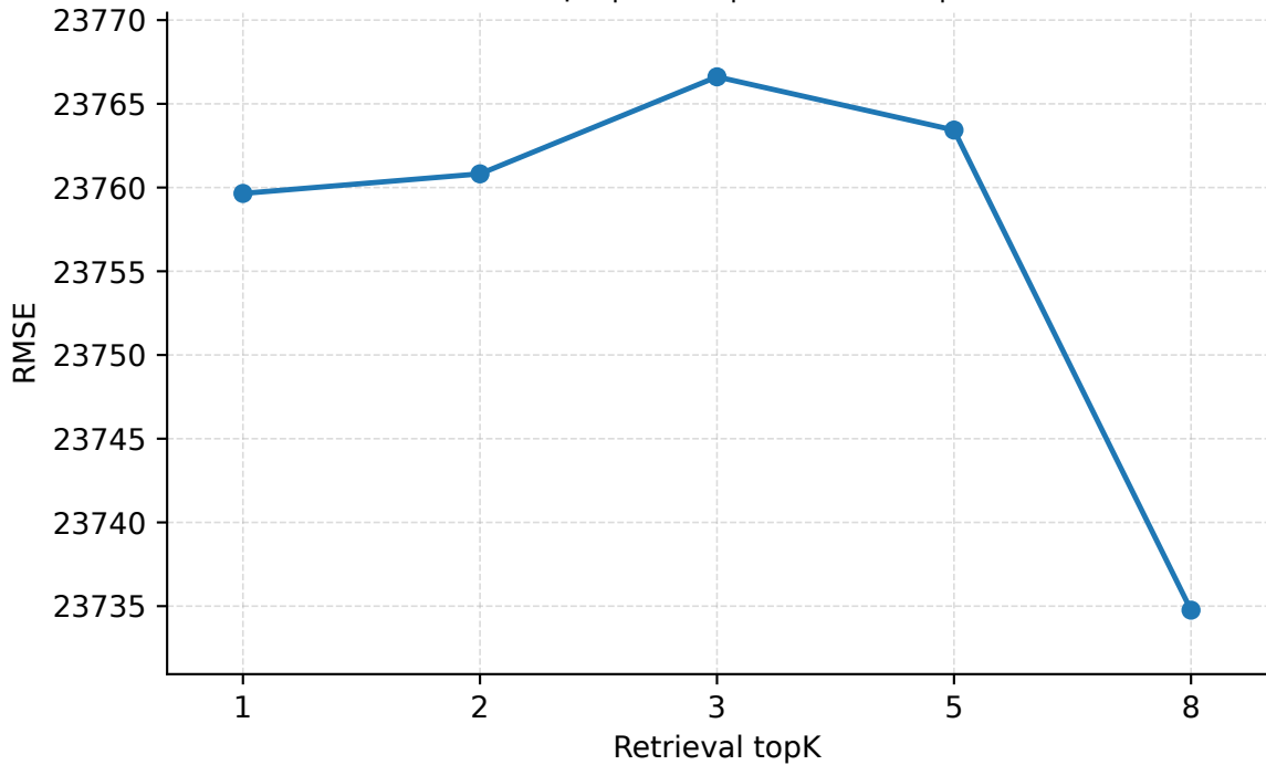
Retrieval topK | Geant | PredLen=15 | RMSE
