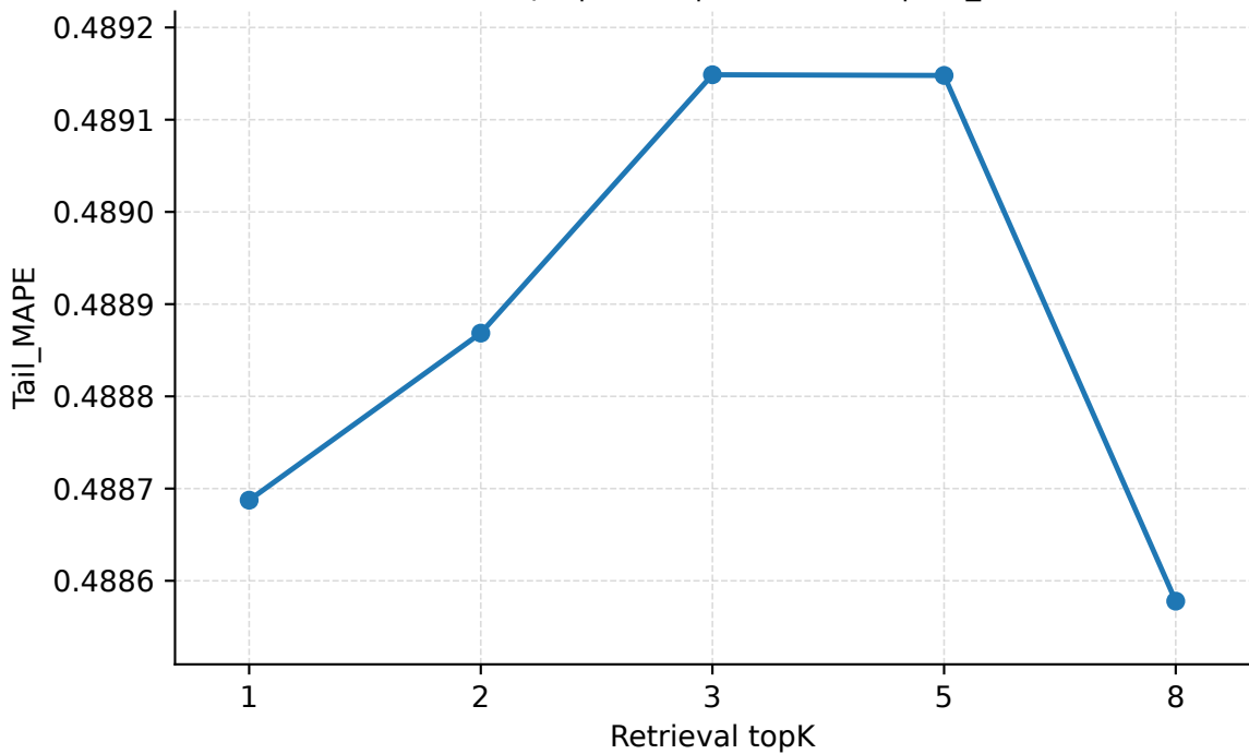
Retrieval topK | Geant | PredLen=15 | Tail_MAPE
