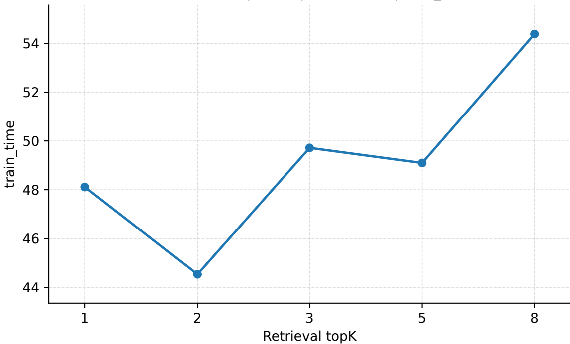
Retrieval topK | Geant | PredLen=15 | train_time
