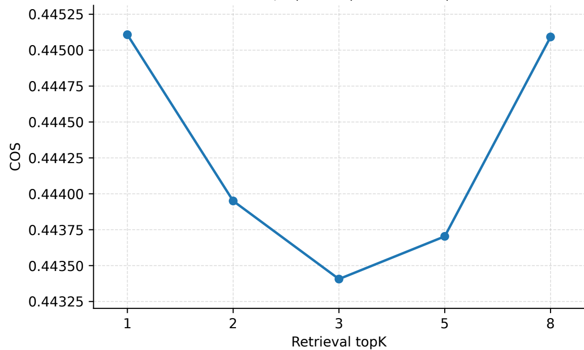
Retrieval topK | Geant | PredLen=20 | COS
