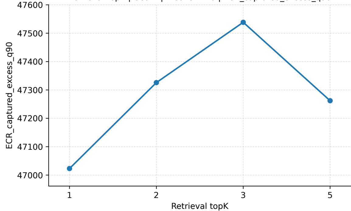
Retrieval topK | Geant | PredLen=20 | ECR_captured_excess_q90
