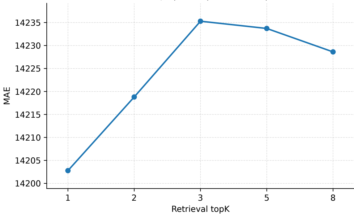
Retrieval topK | Geant | PredLen=20 | MAE
