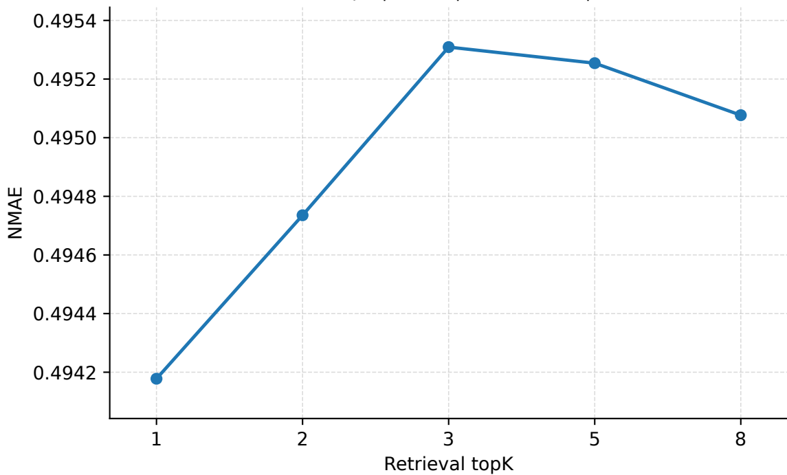
Retrieval topK | Geant | PredLen=20 | NMAE
