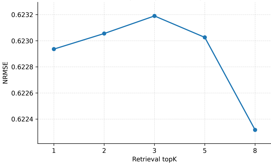
Retrieval topK | Geant | PredLen=20 | NRMSE
