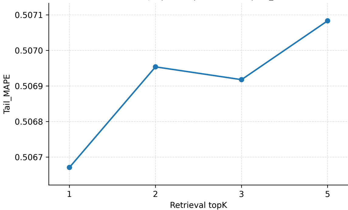
Retrieval topK | Geant | PredLen=20 | Tail_MAPE
