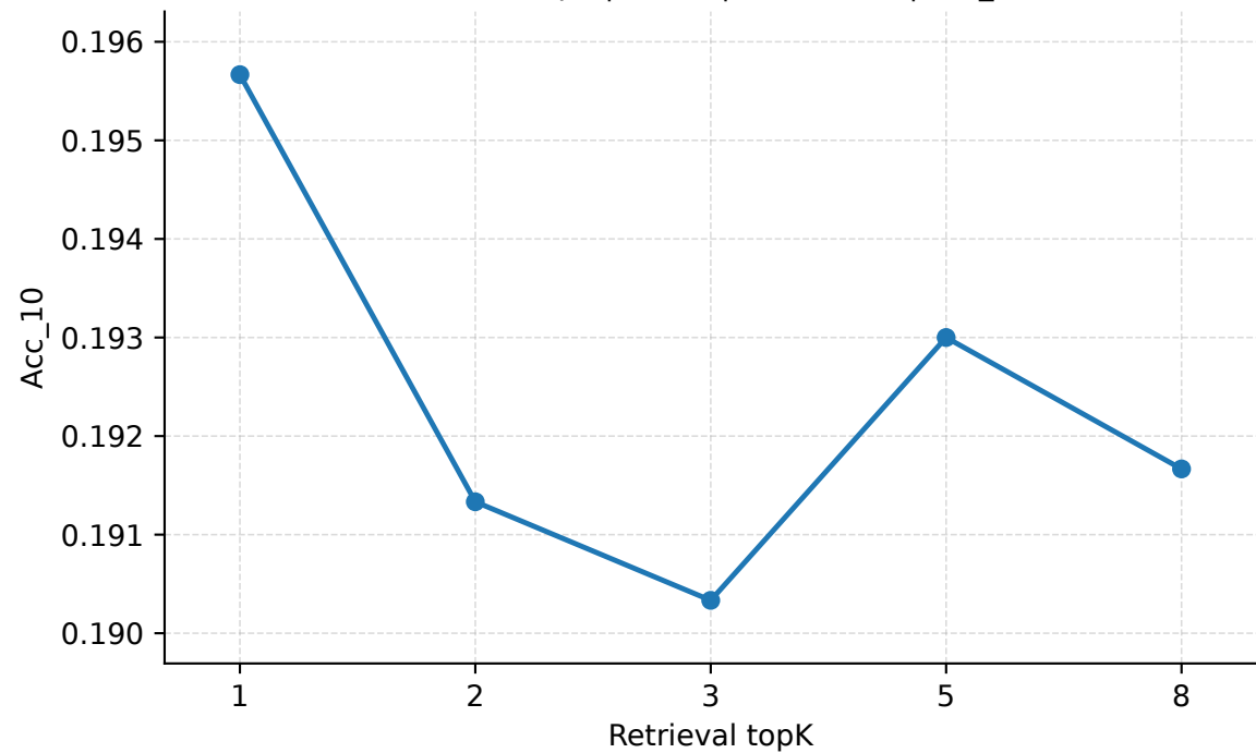
Retrieval topK | Geant | PredLen=5 | Acc_10
