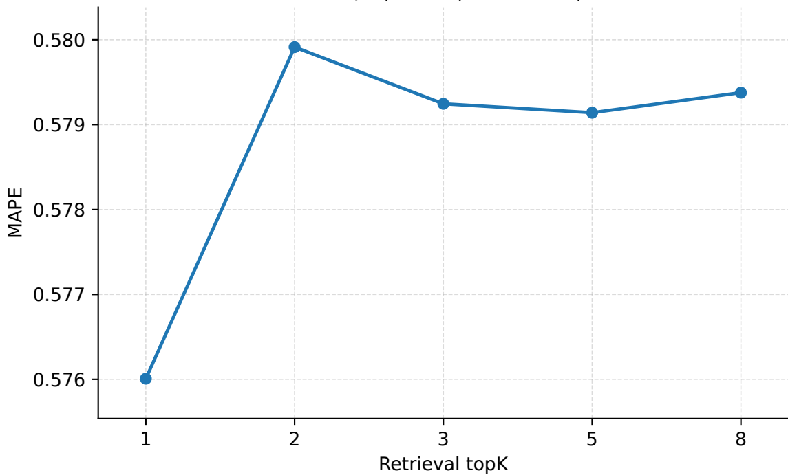
Retrieval topK | Geant | PredLen=5 | MAPE
