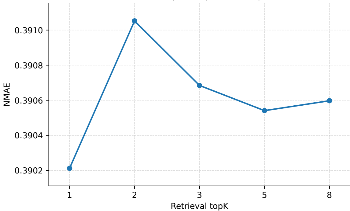
Retrieval topK | Geant | PredLen=5 | NMAE
