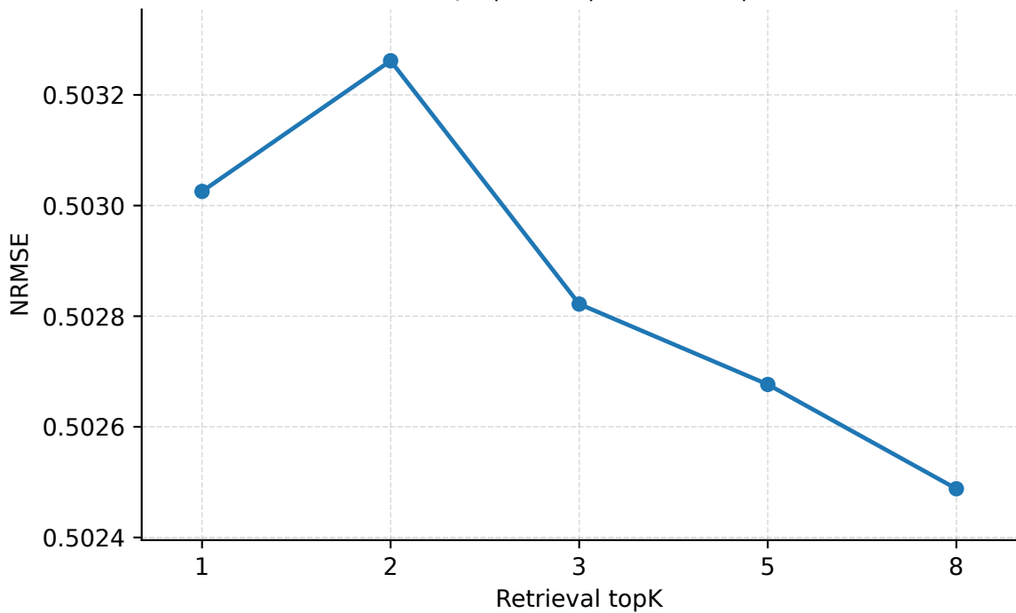
Retrieval topK | Geant | PredLen=5 | NRMSE
