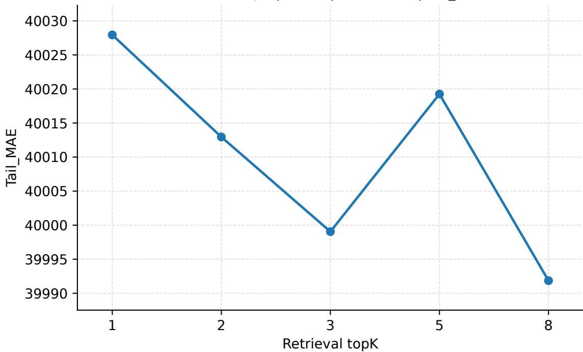
Retrieval topK | Geant | PredLen=5 | Tail_MAE
