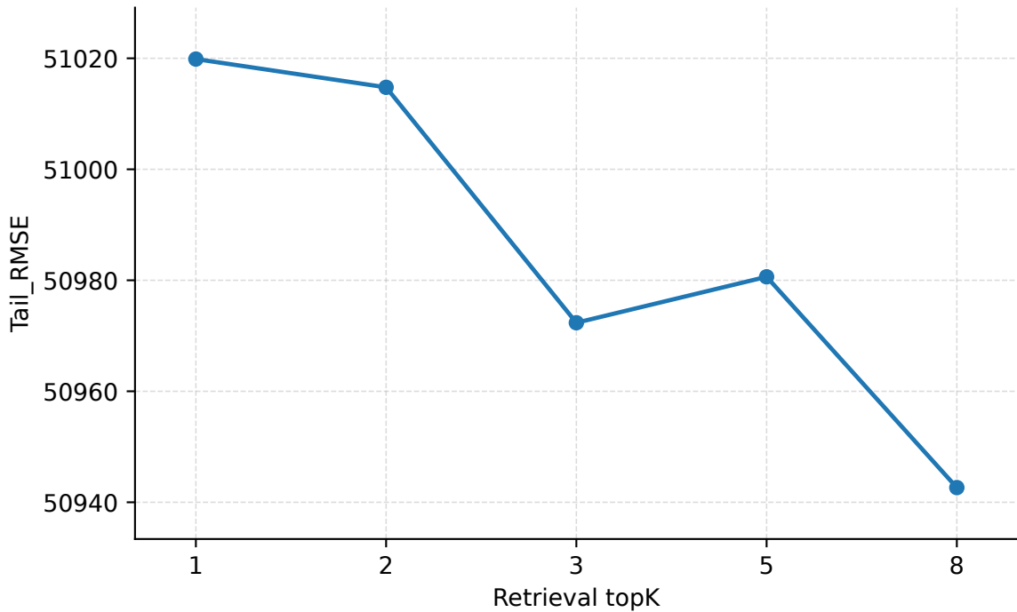
Retrieval topK | Geant | PredLen=5 | Tail_RMSE
